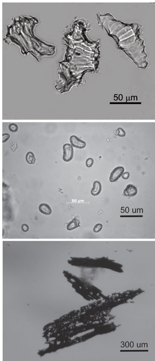
Fig. 3. Microfossils found in soils in Amazonia that can document human activity and environmental changes. The top panel shows phytoliths from the tree Licania micrantha Miq. (Chrysobalanaceae), which are diagnostic to at least the genus level (Piperno and McMichael, 2023) (Photo: Dolores Piperno). The middle panel shows starch grains of Phaseolus vulgaris L. (beans) (Photo: Dolores Piperno). The bottom panel shows charcoal isolated from Amazonian soils (Photo: Crystal McMichael).
