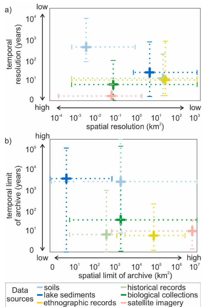
Fig. 4. The spatial and temporal characteristics of data sources used to assess past human activities and vegetation change. (a) Each type of archival material color-coded and plotted in relation to its spatial resolution (the highest possible sampling frequency of archival material across space) and temporal resolution (the highest possible sampling frequency of archival material through time). (b) The types of archival materials are plotted in relation to their spatial and temporal limits (the total amount of space or time captured within an archive). Dotted lines indicate the potential range of resolution/limit achieved from each data source. Crosses are centered on the most common resolution/limit achieved by sampling efforts on the data sources in Amazonia.
